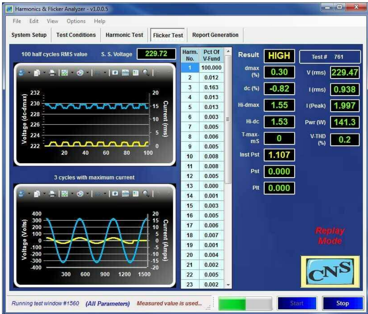
Figure 27 Modulation at 8.77 Hz
