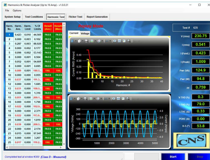
Figure 34 The Class-D test screen
