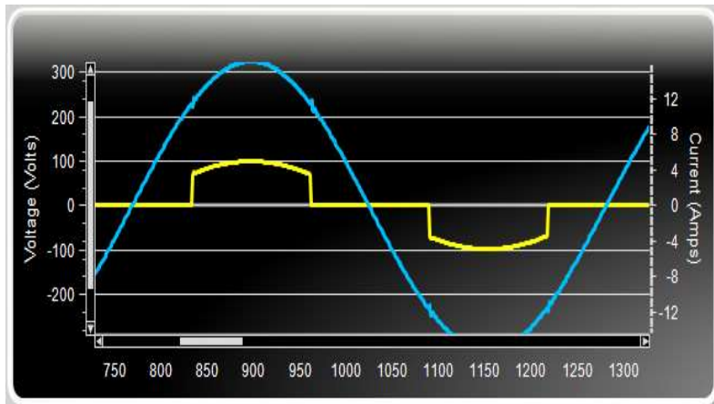
Figure 20 The "zoomed in" waveform graph display
