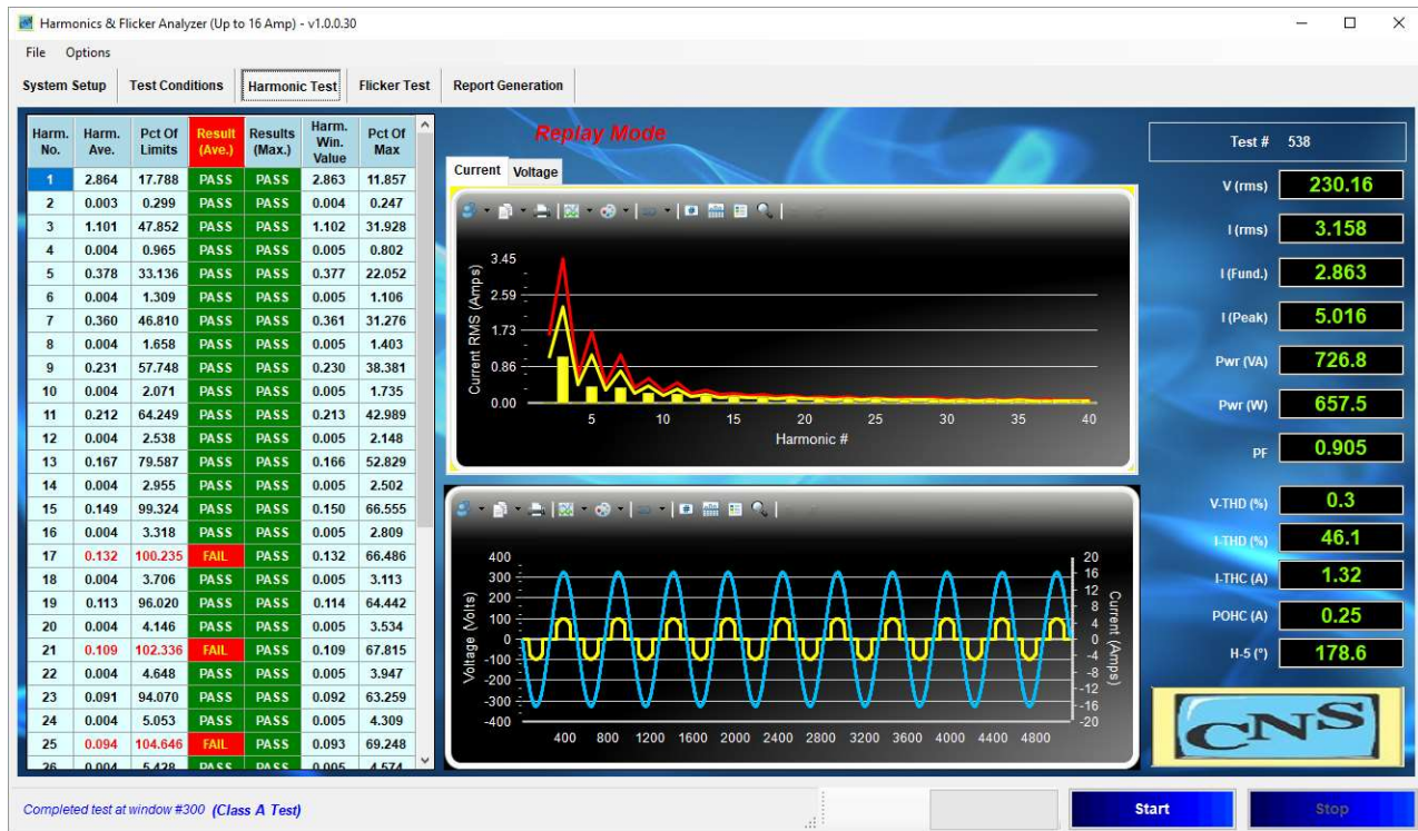
Figure 18 The Class-A "FAIL" display, "stretched" to include all data columns
