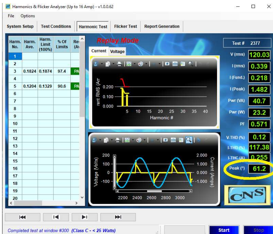
Figure 32 Lighting product < 25 Watt that meets the waveform criteria
