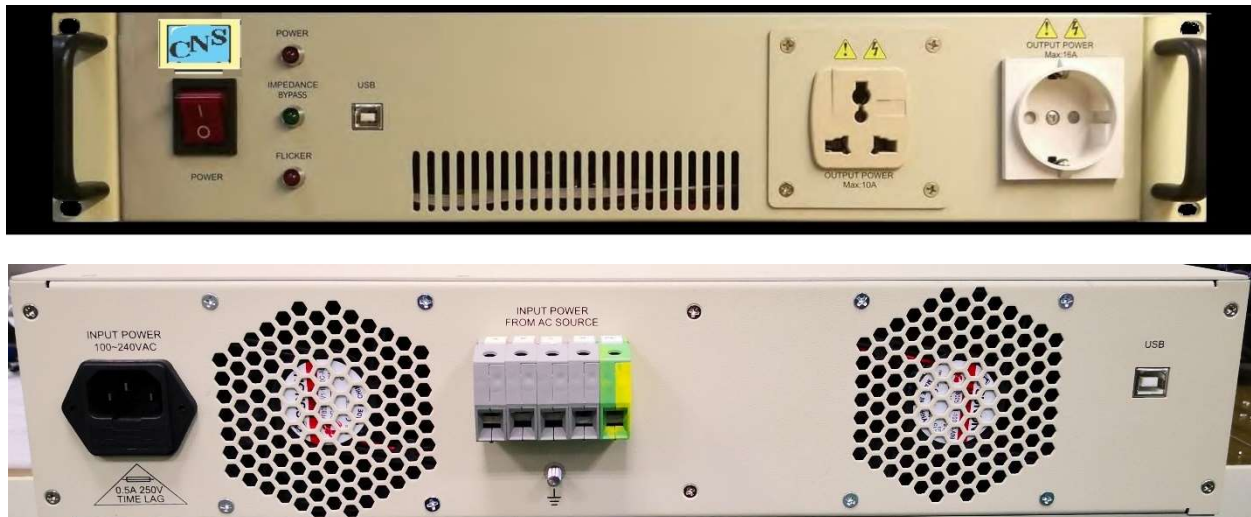
Figure 48 The 19" form factor HFA-1/3-19 box front and rear panel
