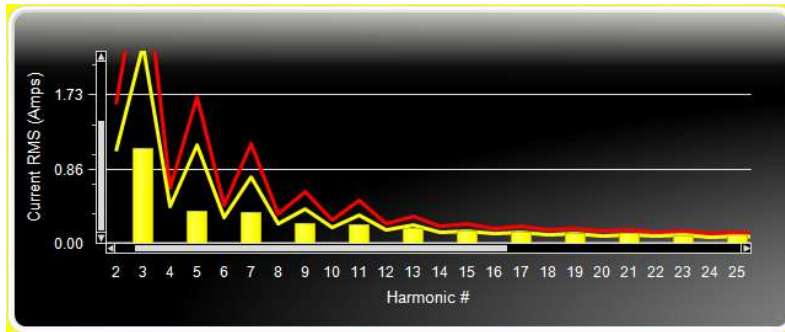
Figure 19 The "zoomed in" current spectrum
