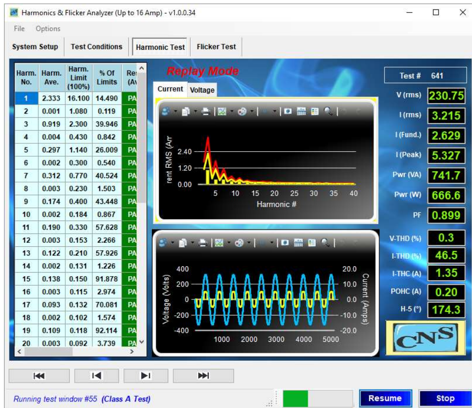
Figure 39 The 1.5 sec filtered data – averaged over the first 55 measurement windows of the test.
