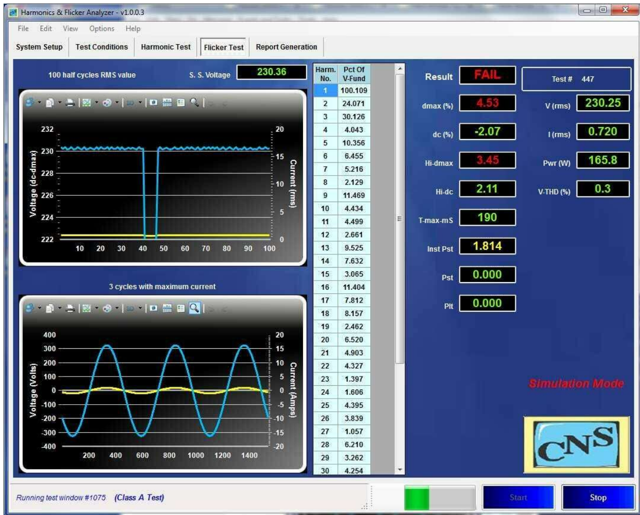
Figure 26 dmax exceeding the limit, and T-max of 190 ms
