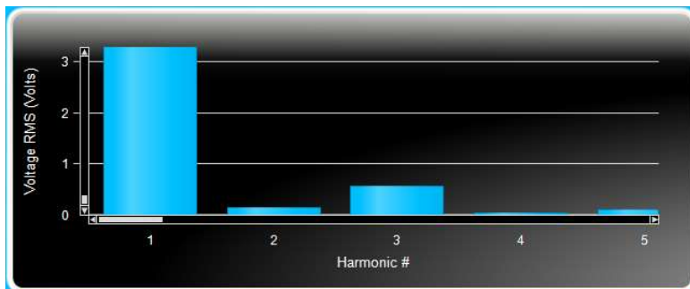
Figure 21 The voltage spectrum (distortion) in detail
