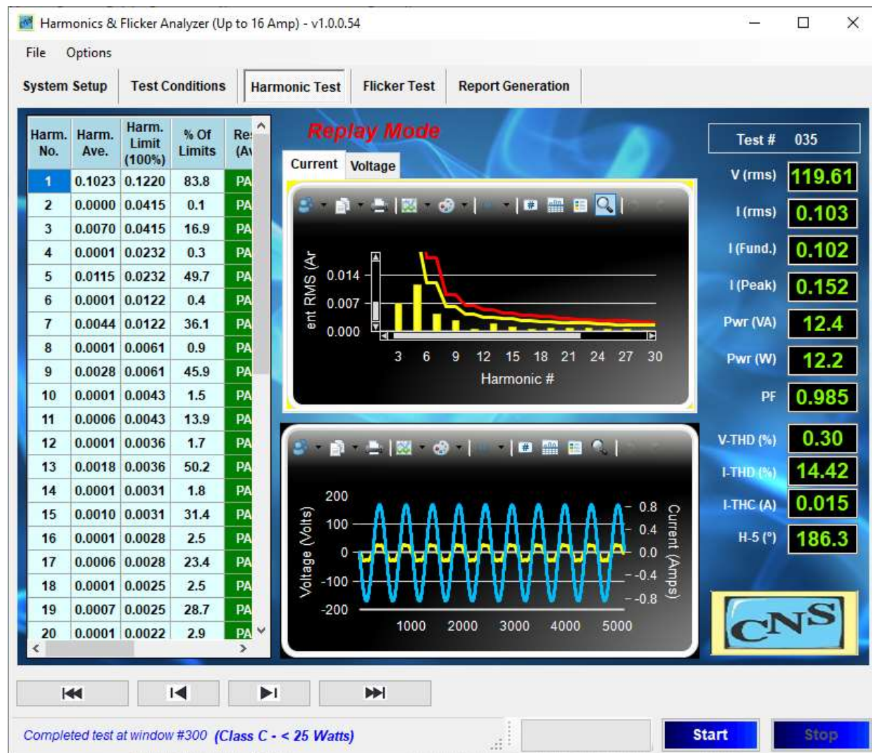
Figure 31 Lighting < 25 Watt meeting Table-3
