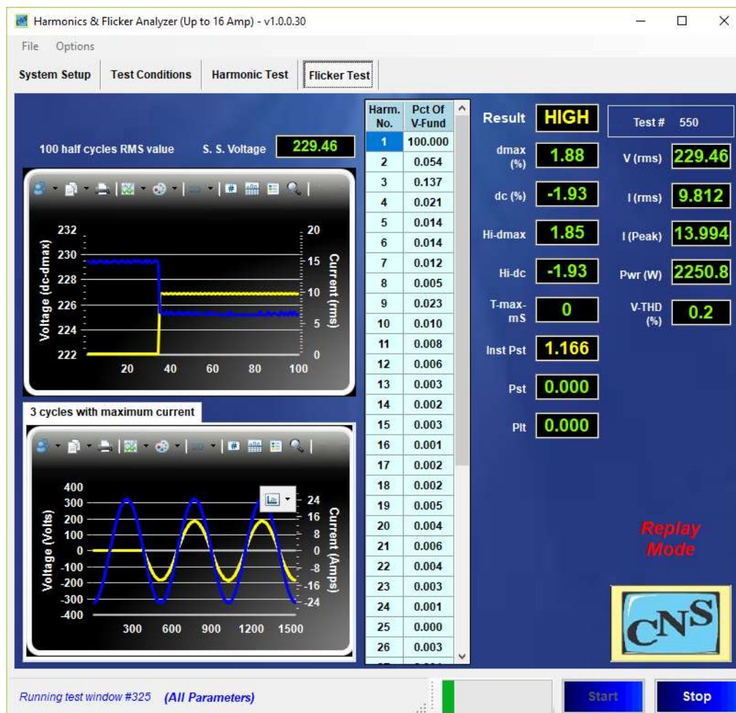
Figure 24 The Flicker test screen
