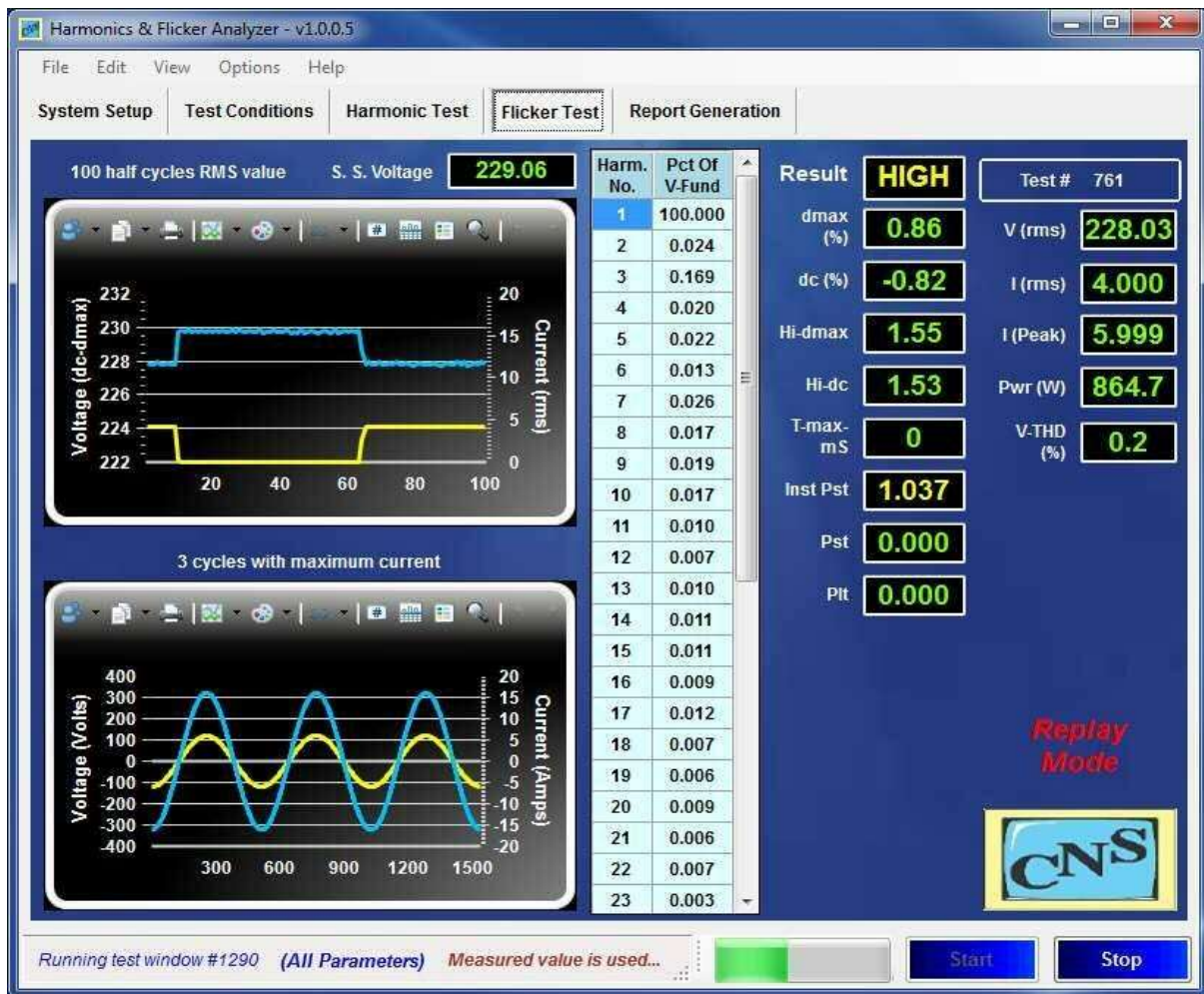
Figure 25 Flicker test with 0.917 Hz modulation
