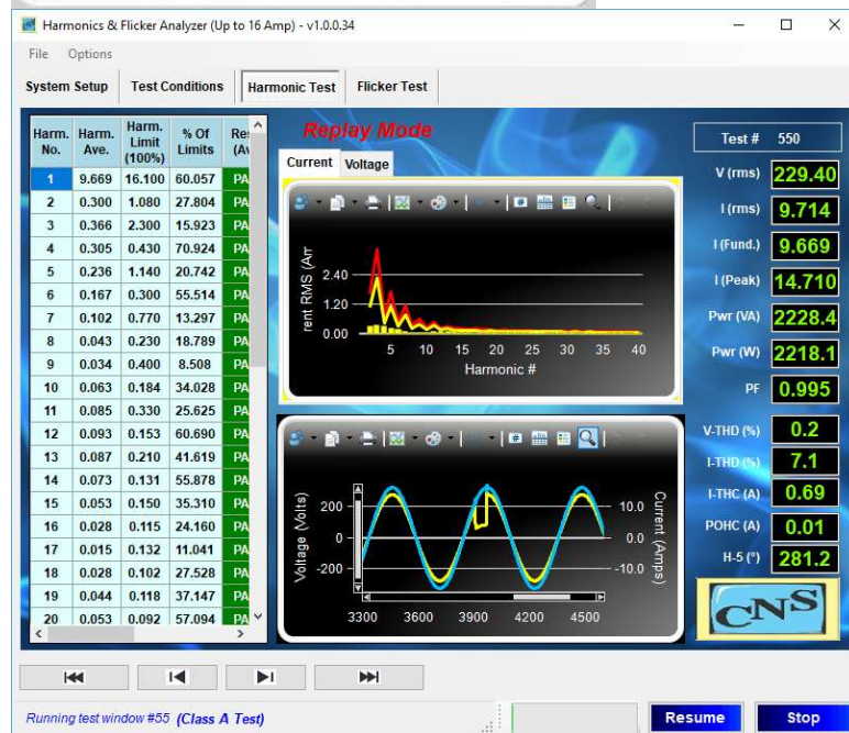
Figure 43 Short glitch
