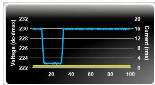
Figure 42 180 ms voltage drop-out
