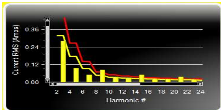
Harmonic Spectrum
