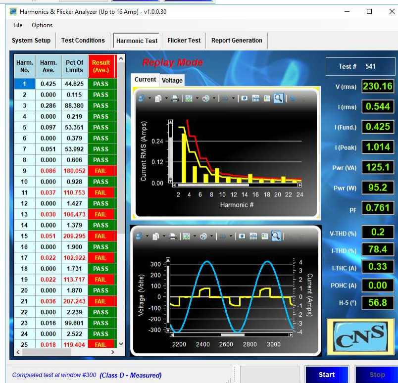
Figure 35 The Class-D display with “zoomed in” graphs
