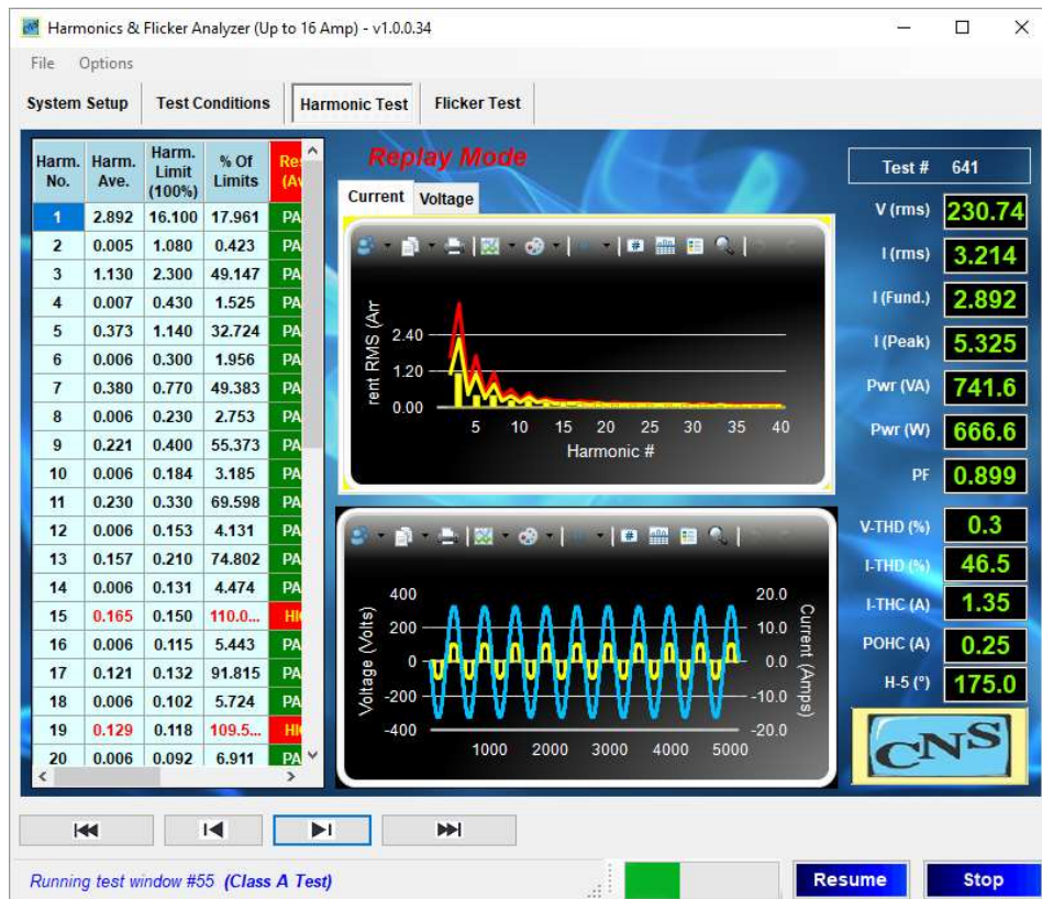
Figure 40 The same unfiltered measurement window # 55
